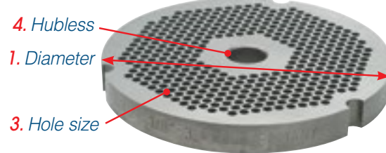
Enterprise Style HUBLESS Plate Pictured
